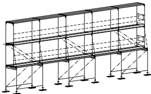
3D - Skizze
